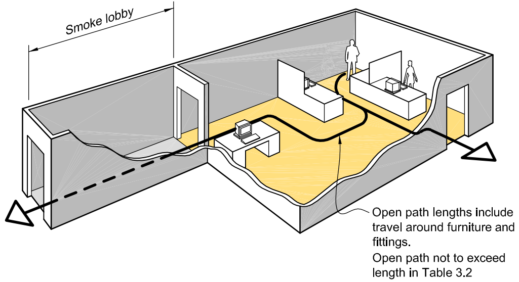
Figure 3.7 Length of open paths Paragraph 3.4.2 c)
