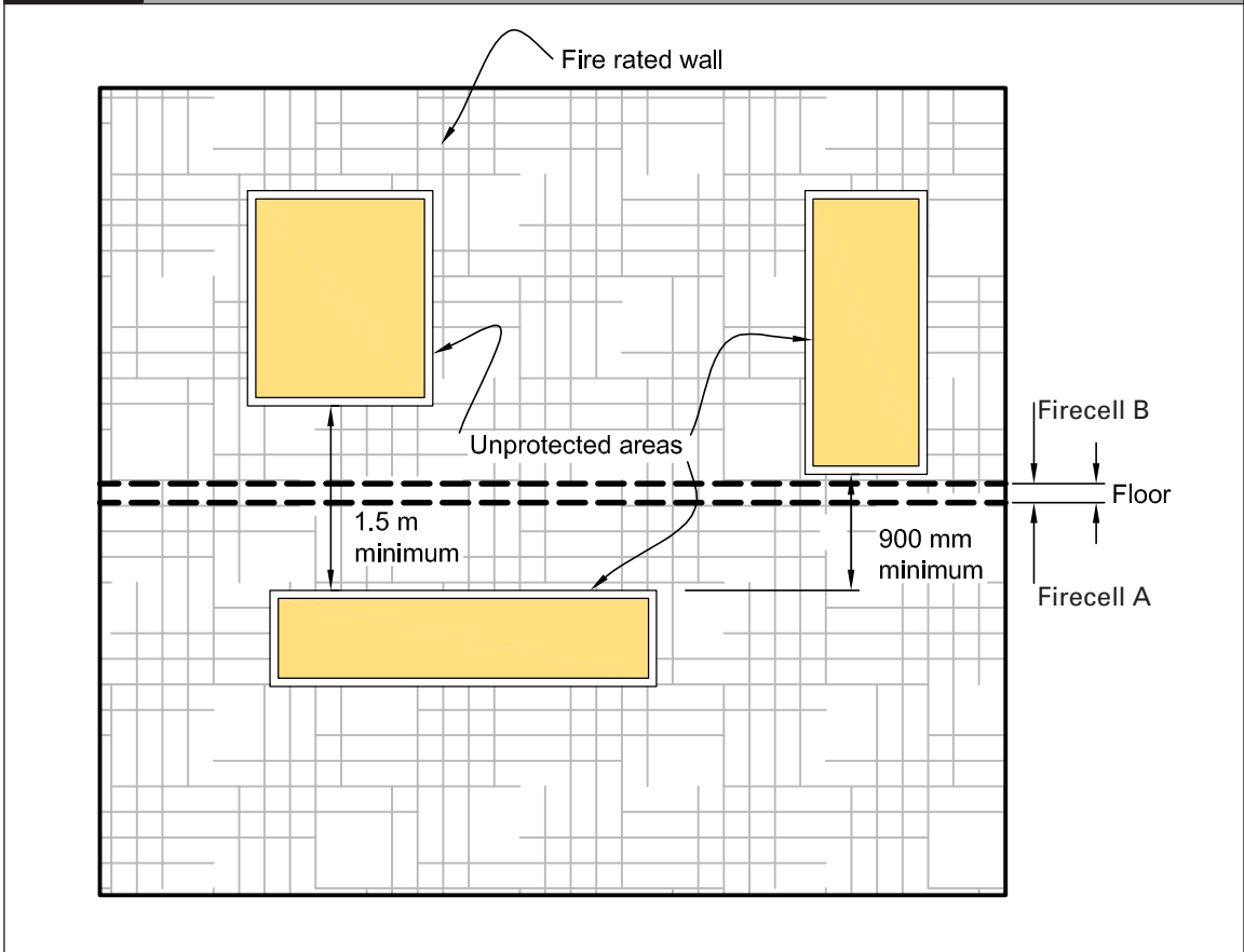
Figure 5.7 Separation of unprotected areas Paragraph 5.7.11
